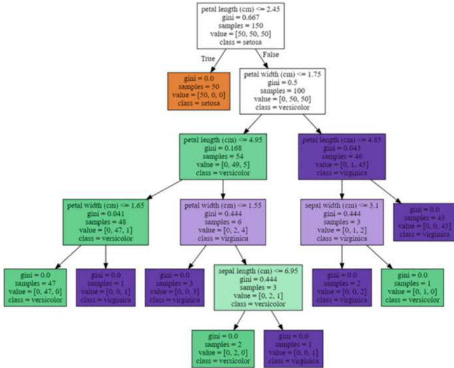
Fig. 4.4 Tree generated by fitting the Iris dataset with CART
