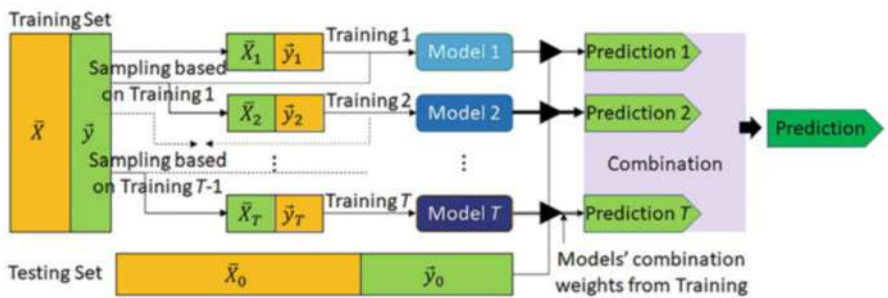
Fig. 9.8 Procedure of boosting
