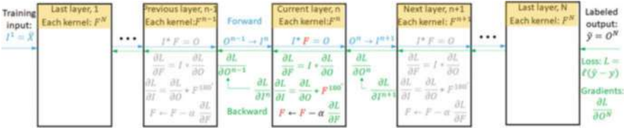
Fig. 8.2 Backpropagation through convolution layers
