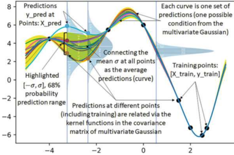
Fig. 6.5 Conceptual illustration of the Gaussian process
