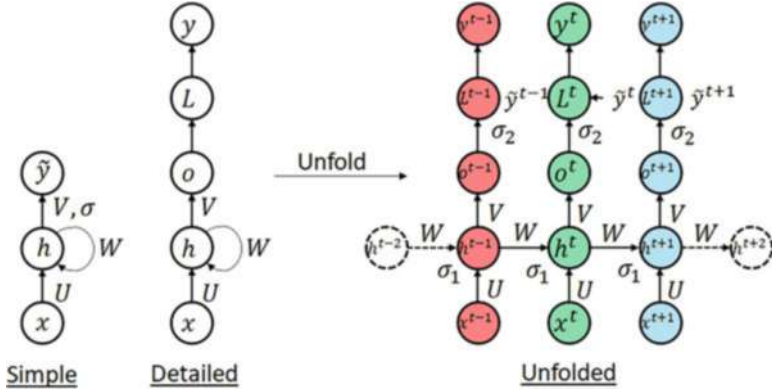
Fig. 8.10 Structure and workflow of RNN
