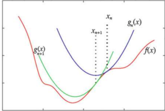
Fig. A.1 Approximation for optimization
