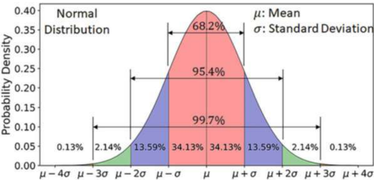
Fig. 12.1 Three sigma: 99.7% of the data are within three standard deviations of the mean
