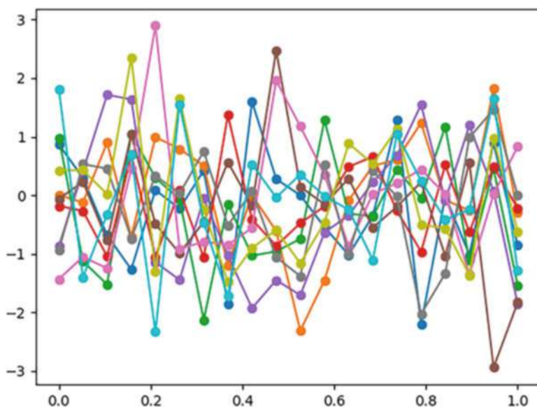
Fig. 6.6 Samples from a 20D Gaussian without kernel smoothing
