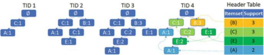
Fig. 13.5 Generation of the FP tree
