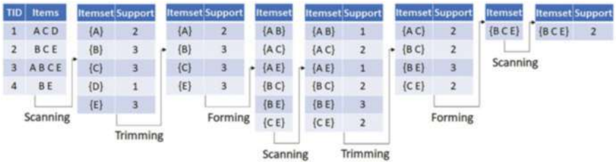
Fig. 13.3 Illustration of the implementation of Apriori with an example
