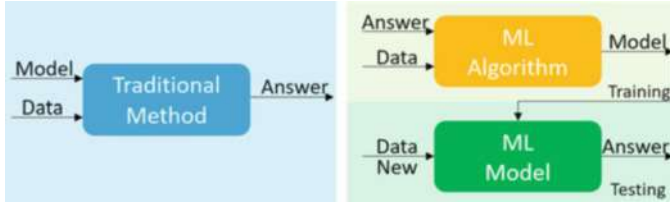
Fig. 1.3 Workflows of physics-based methods (left) and data-driven methods (right)
