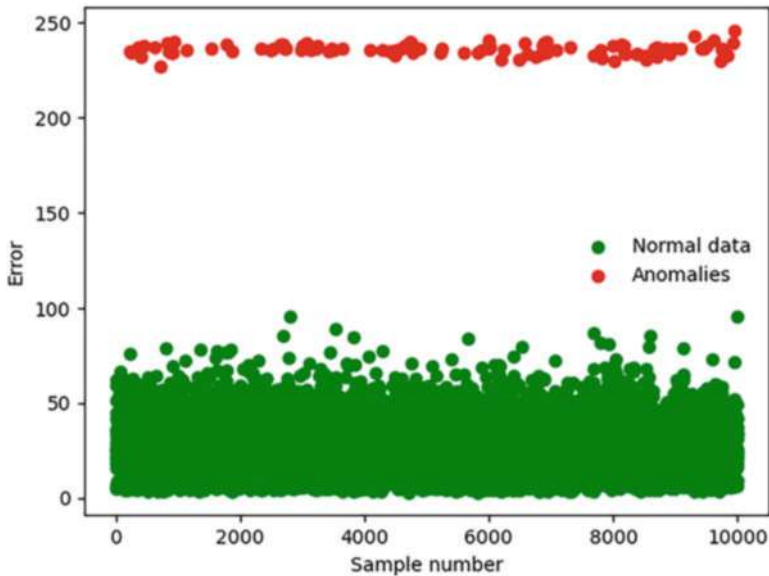
Fig. 12.6 Results for using autoencoder for anomaly detection
