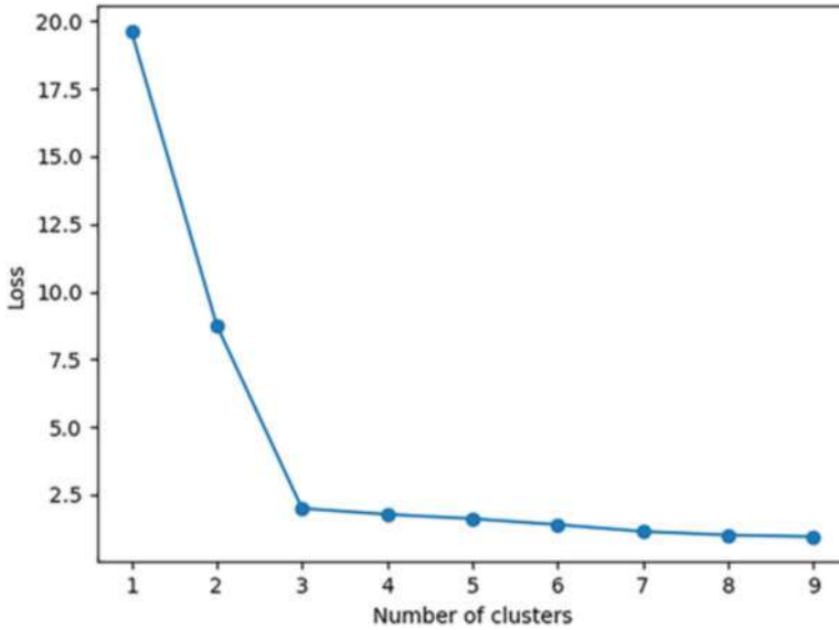
Fig. 10.3 Loss vs. number of clusters
