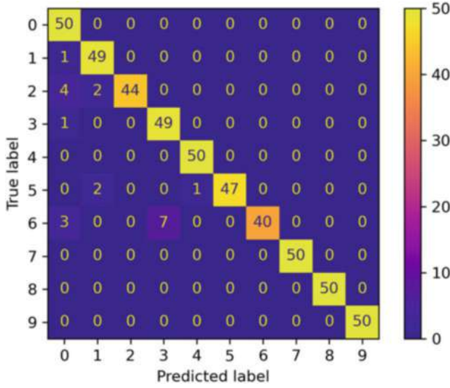
Fig. A.5 Confusion matrix for multiclass classification problem
