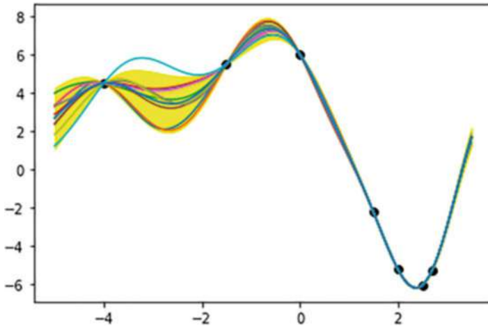
Fig. 6.10 Final results of Gaussian process analysis
