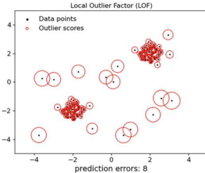
Fig. 12.3 Local outlier factor (LOF)
