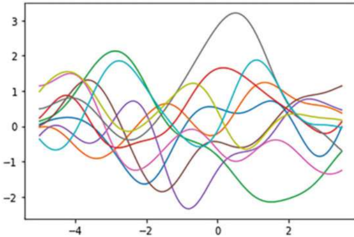
Fig. 6.9 Multivariate Gaussian sampling without relating training data to testing data
