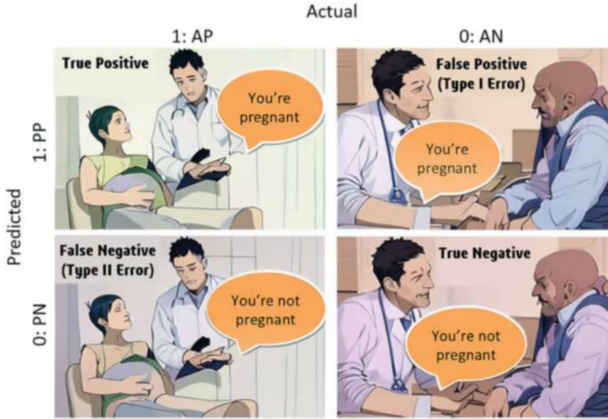
Fig. A.3 Two types of errors
