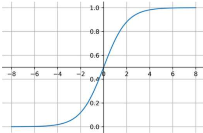
Fig. 3.3 Plot of logistic function
