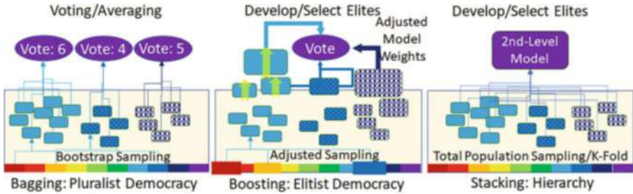
Fig. 9.4 Categories of ensemble learning algorithms
