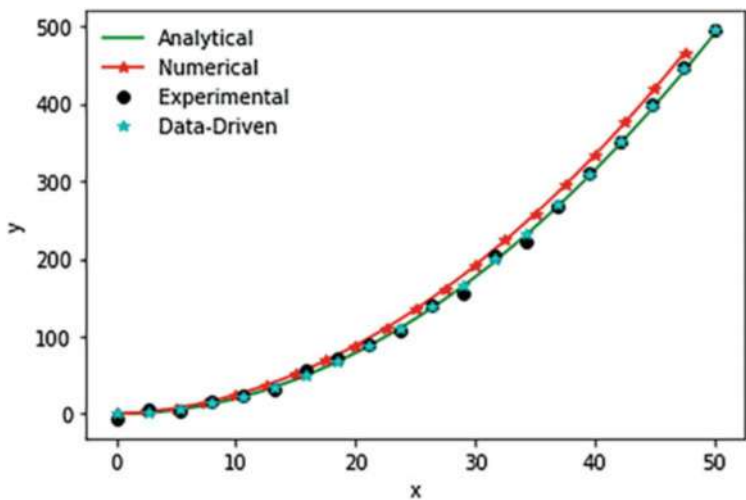
Fig. 1.5 Results of problem-solving using different types of methods
