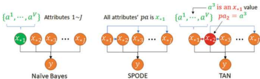
Fig. 6.2 Naïve Bayes and semi-naïve Bayes methods
