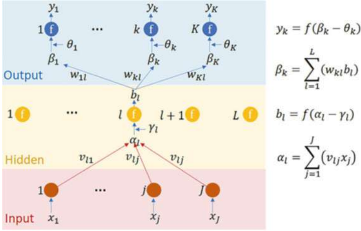
Fig. 7.3 Forward propagation in a 3-layer ANN
