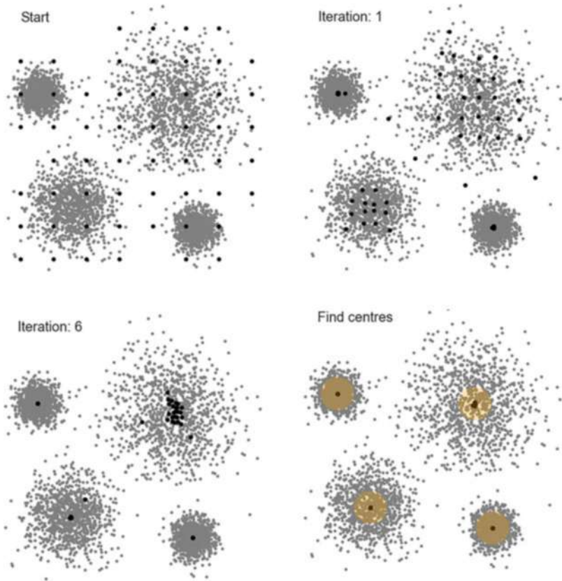
Fig. 10.4 Typical process of mean-shift clustering
