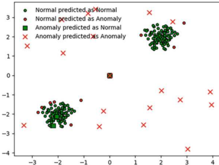
Fig. 12.4 Results of an iForest implementation
