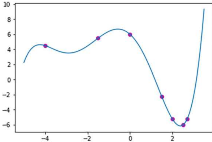
Fig. 6.8 True solution and training data for Gaussian process example
