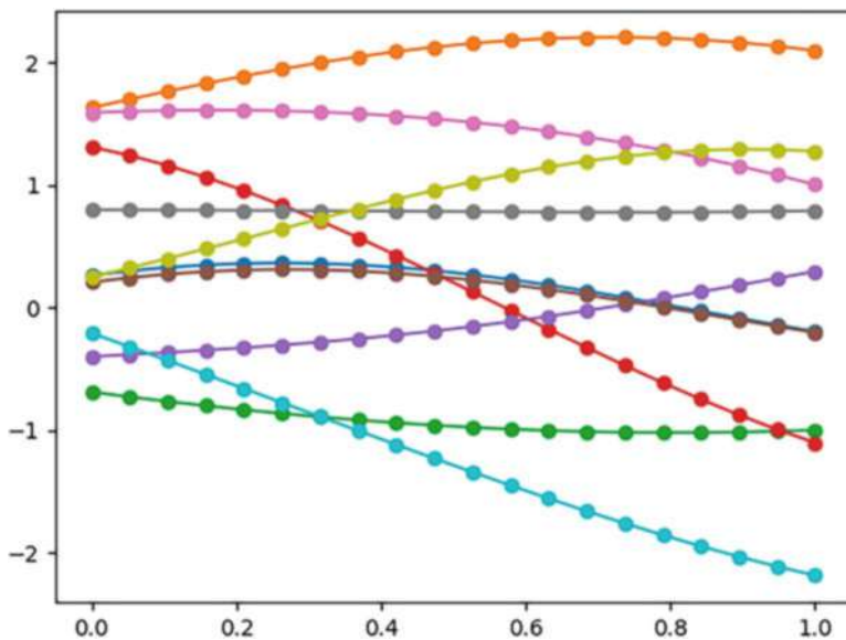
Fig. 6.7 Samples from a 20D Gaussian with kernel smoothing
