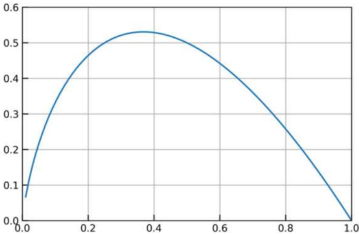
Fig. 4.3 Information entropy function
