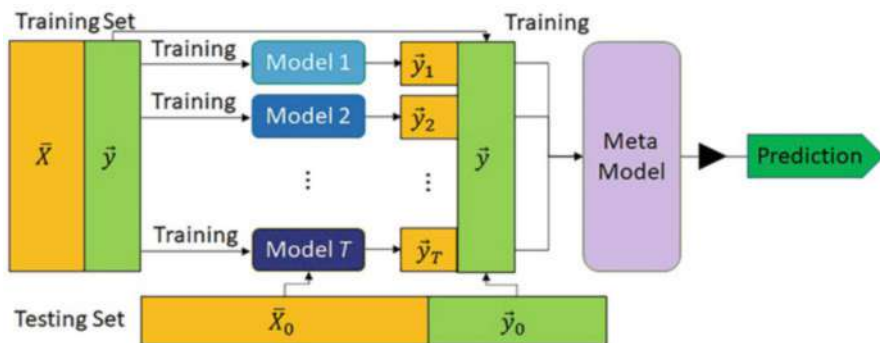
Fig. 9.11 Procedure of stacking
