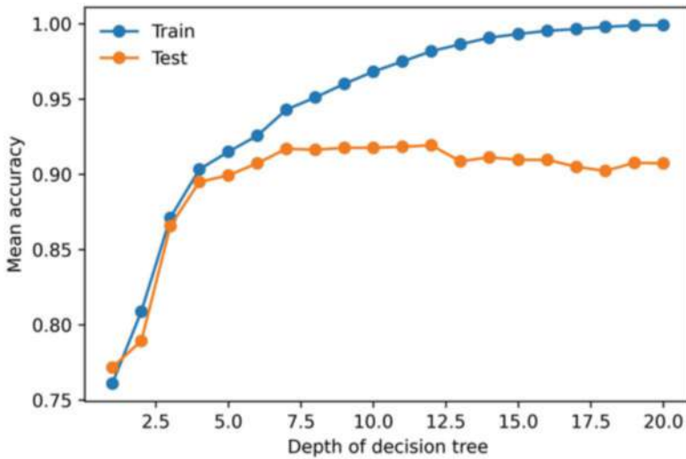
Fig. 4.5 Overfitting in the training of a decision tree (10,000 samples and each with 30 attributes)
