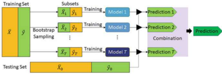
Fig. 9.7 Procedure of bagging
