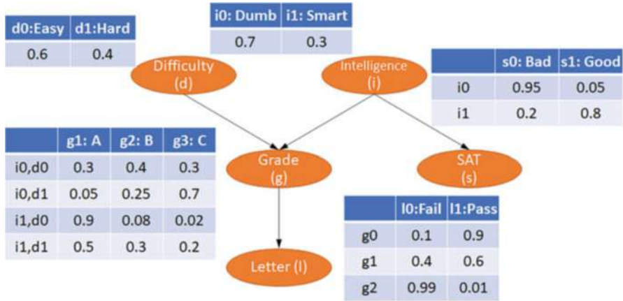
Fig. 6.4 Example for using Bayesian networks
