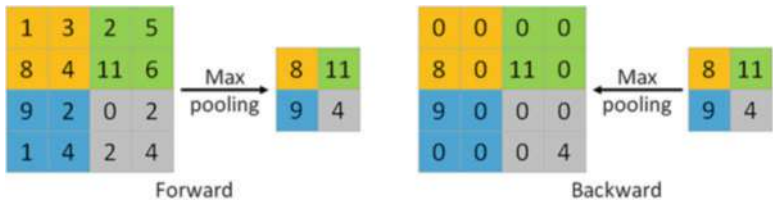
Fig. 8.9 Forward and backward passes in backpropagation of max pooling layer
