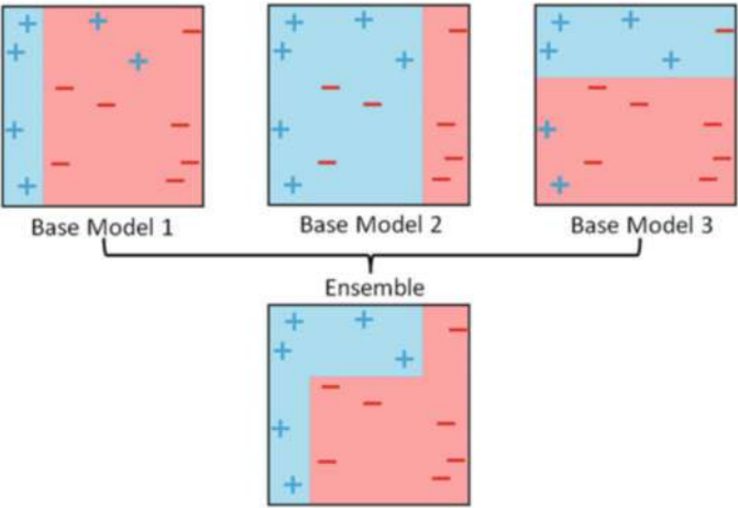
Fig. 9.3 Illustration of ensemble learning process
