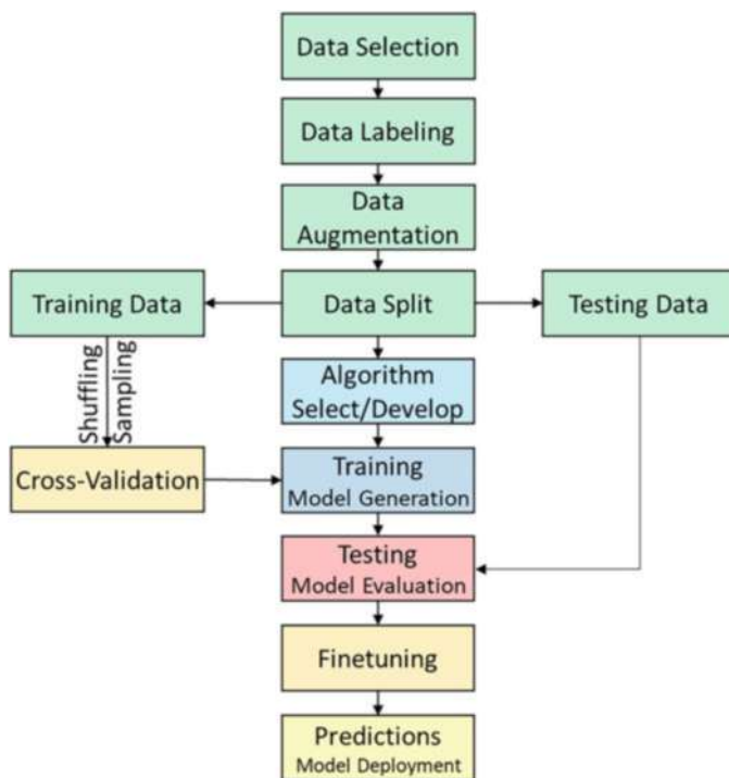
Fig. 1.7 Machine learning (supervised) workflow
