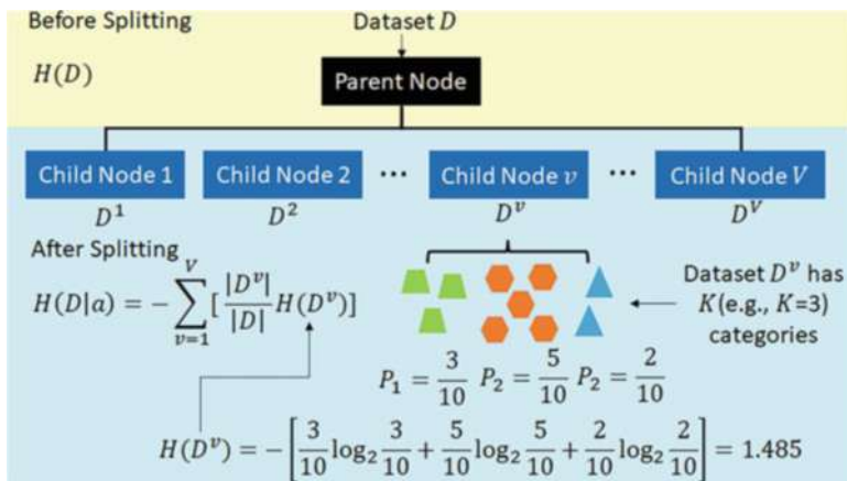
Fig. 4.2 An example for dataset splitting and information entropy change
