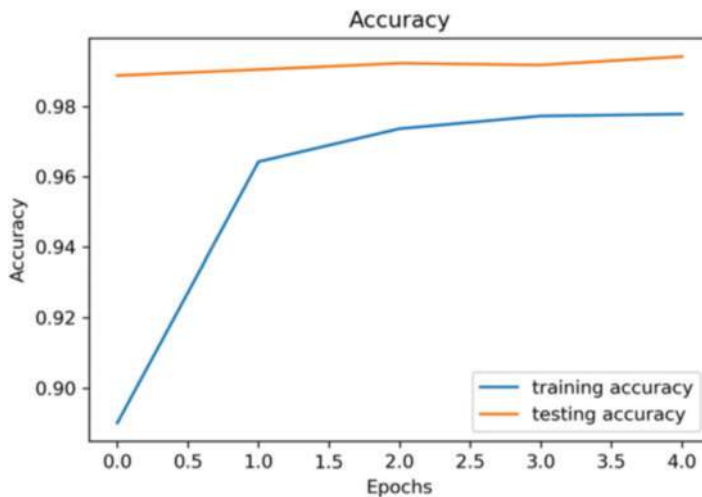
Fig. 2.7 Variation of training and testing accuracy with epochs
