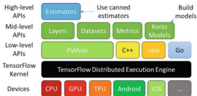
Fig. 2.5 Architecture of TensorFlow
