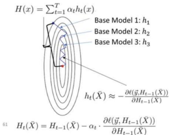
Fig. 9.10 Model update in gradient boosting
