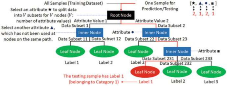
Fig. 4.1 Conceptual illustration of decision tree
