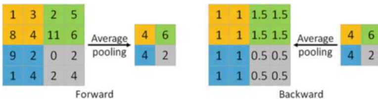
Fig. 8.8 Forward and backward passes in backpropagation of average pooling layer
