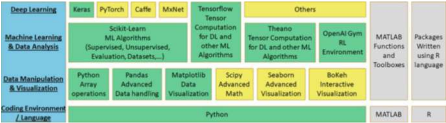
Fig. 2.1 Structure of Python-based AI tools
