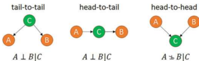
Fig. 6.3 Three basic units in typical Bayesian networks
