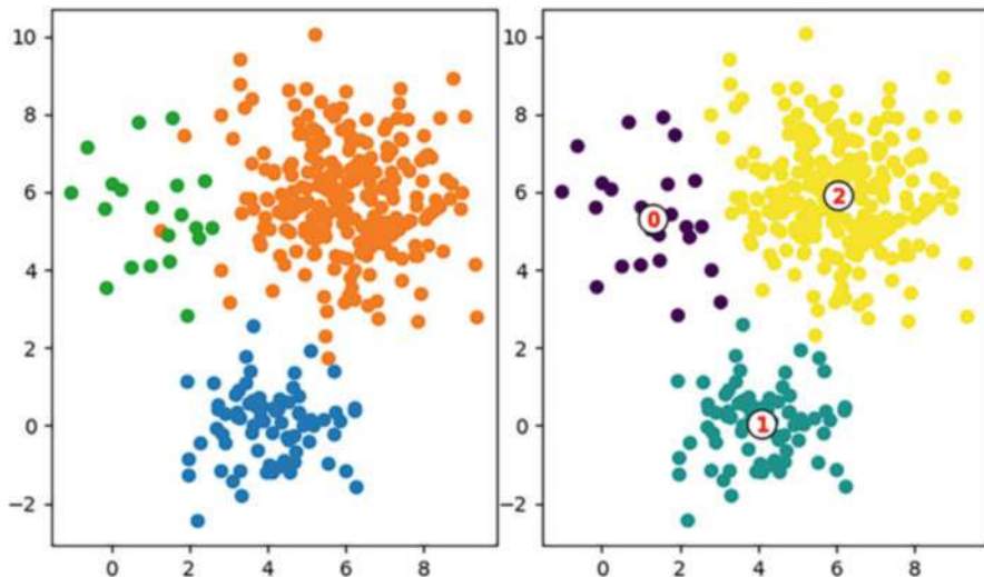
Fig. 10.6 Example of GMM: data generated with three normal distributions and their GMM clustering
