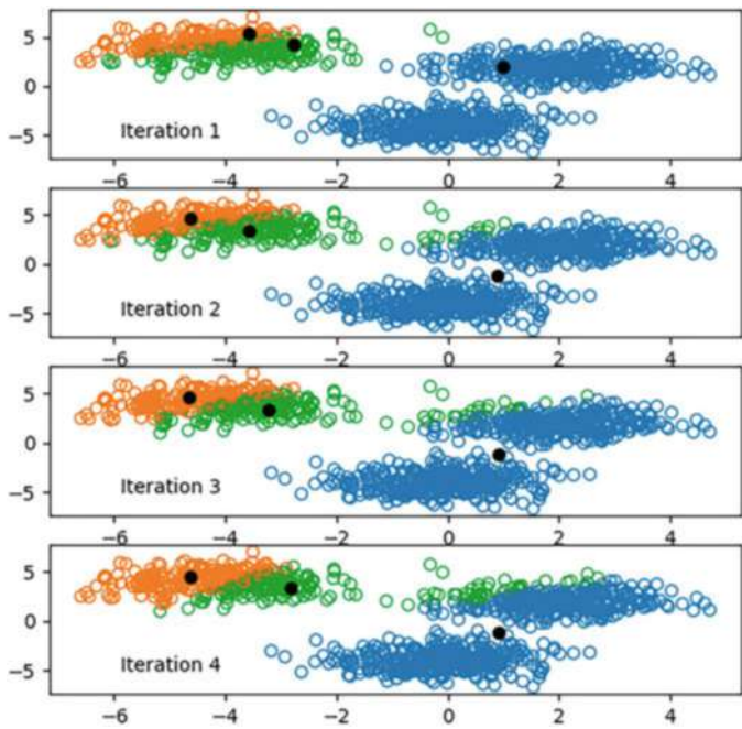
Fig. 10.2 Example of clustering process using K-means with a different initialization
