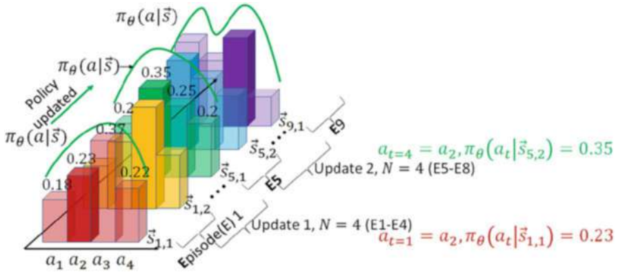
Fig. 15.2 Illustration of policy update in policy-based RL
