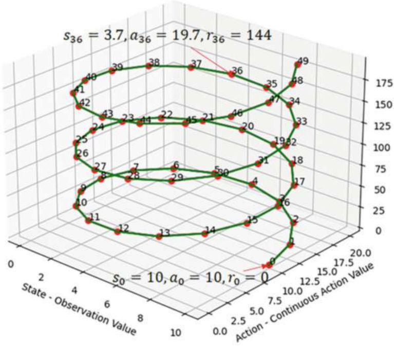
Fig. 15.3 Trajectory of an episode in RL learning
