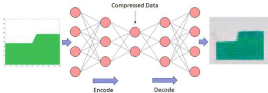
Fig. 12.5 Illustration of autoencoder
