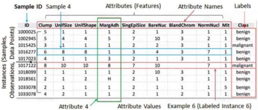
Fig. 1.6 Structure of data for (supervised) machine learning
