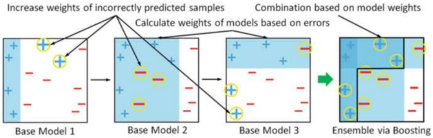
Fig. 9.9 Example of boosting
