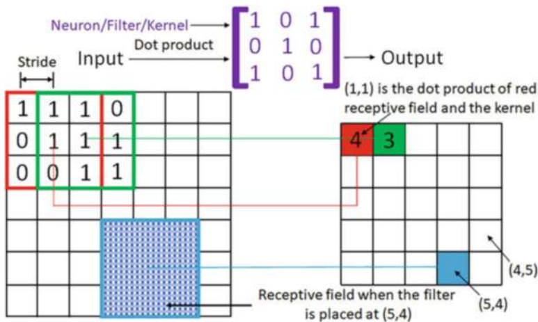
Fig. 8.3 Schematic of the application of a kernel to a 2D image (2D array)
