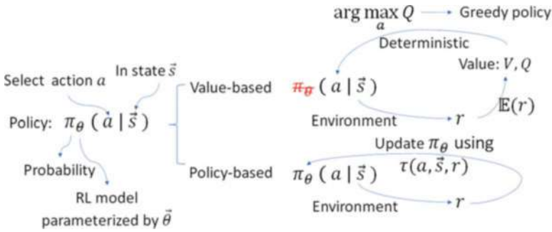
Fig. 15.1 Value-based RL vs. policy-based RL
