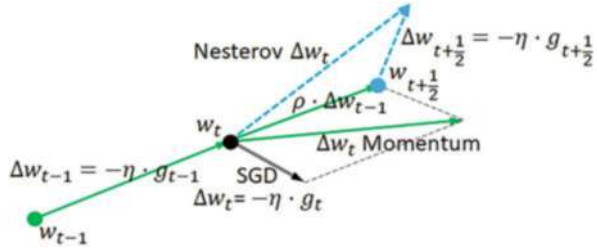
Fig. 8.11 Gradient descent method with manual learning rate
