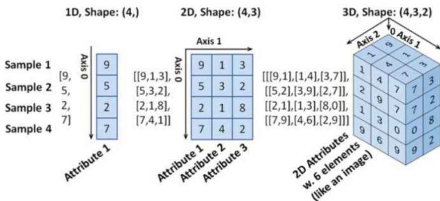
Fig. 2.2 Visualization of Python arrays
