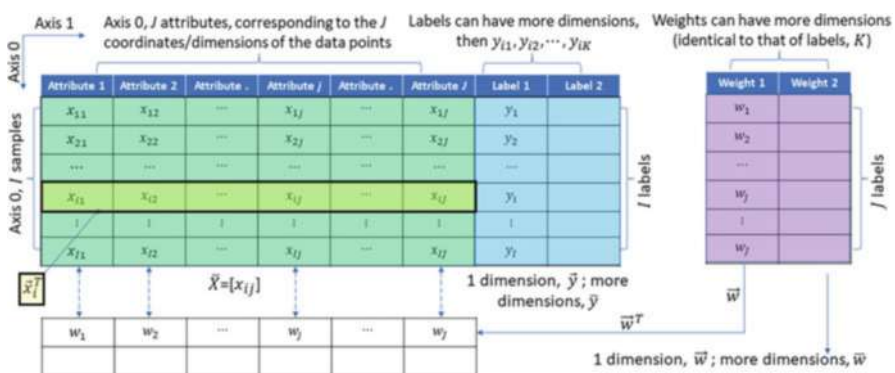
Fig. 3.1 Illustration of general data structure
