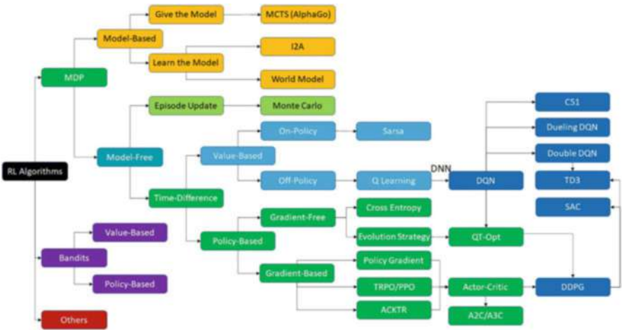
Fig. 14.3 Overview of popular RL algorithms
