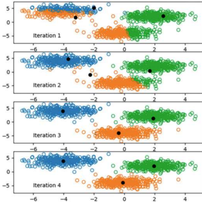
Fig. 10.1 Example of clustering process using K-means
